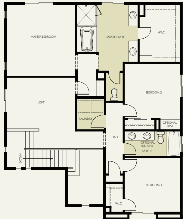
AMERICAN TRADITIONAL • CRAFTSMAN • FARMHOUSE 2 ND FLOOR
